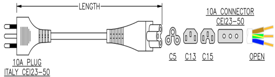
DIMENSIONS 10A PLUG ITALY CEI23-50
