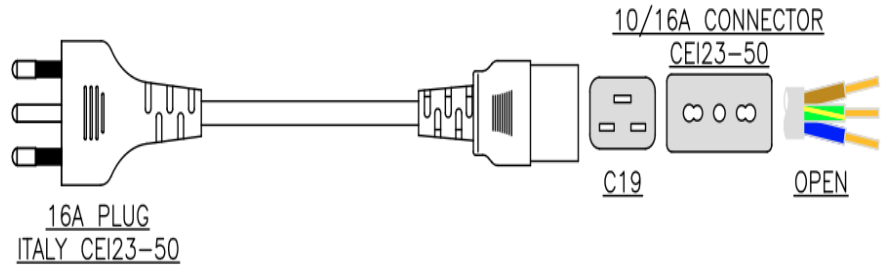
DIMENSIONS 16A PLUG ITALY CEI23-50
