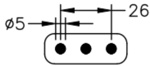
DIMENSIONS 16A PLUG ITALY CEI23-50
