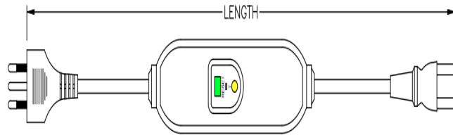
DIMENSIONS 10A PLUG ITALY CEI23-50
