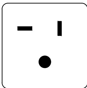
NEMA 6-20P (PLUG SIDE)
