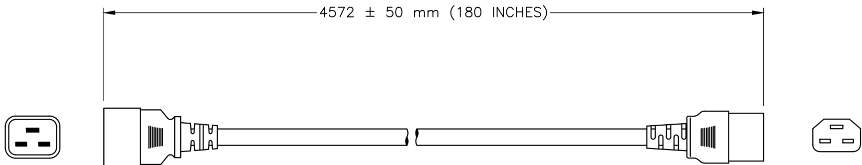
IEC 60320, C20 (ROTATED 90°)
