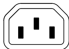
IEC 60320 C14 (PLUG SIDE)
