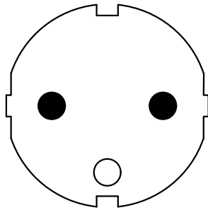
SCHUKO CEE7 (PLUG SIDE)
