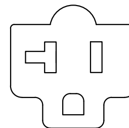
NEMA 5-15/20R (CONNECTOR SIDE)
