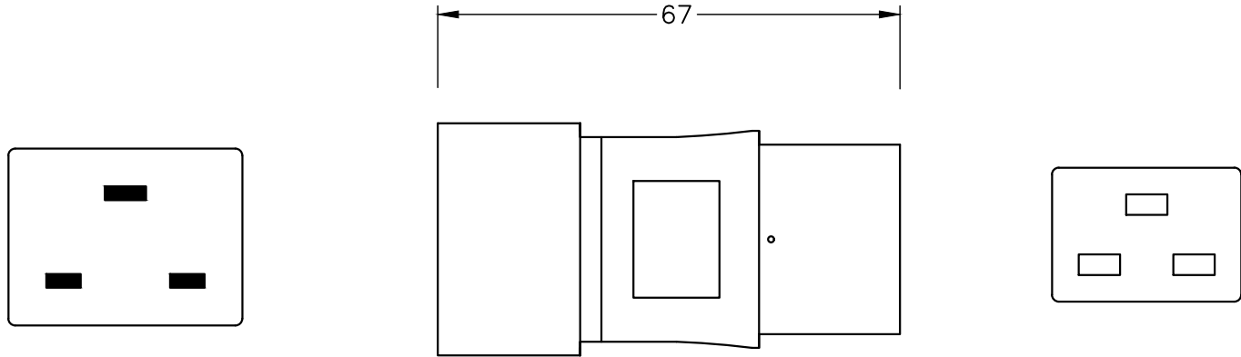
IEC 60320 C20 (PLUG SIDE)
