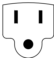
NEMA 5-15P (PLUG SIDE)
